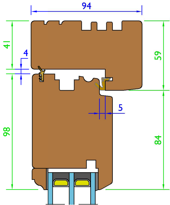
Section A-A - Head Detail (Scale 1:2)
