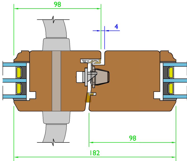
Thumb Bolt Lock Option - (Scale 1:2)
