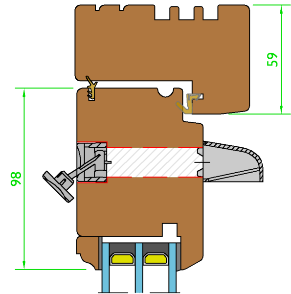
Sash Vent Option (Slide In/Canopy out) - (Scale 1:2)
