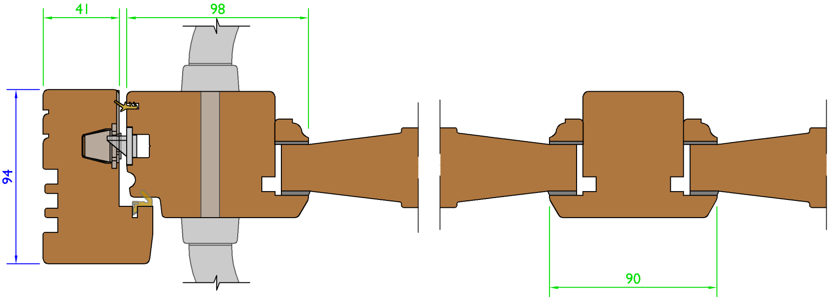
Section B-B - Cill Detail (Scale 1:2)
