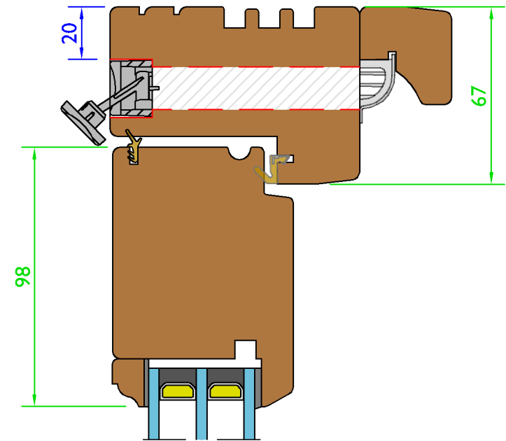
Frame Vent Option (Slide In/Grille Out) - (Scale 1:2)
