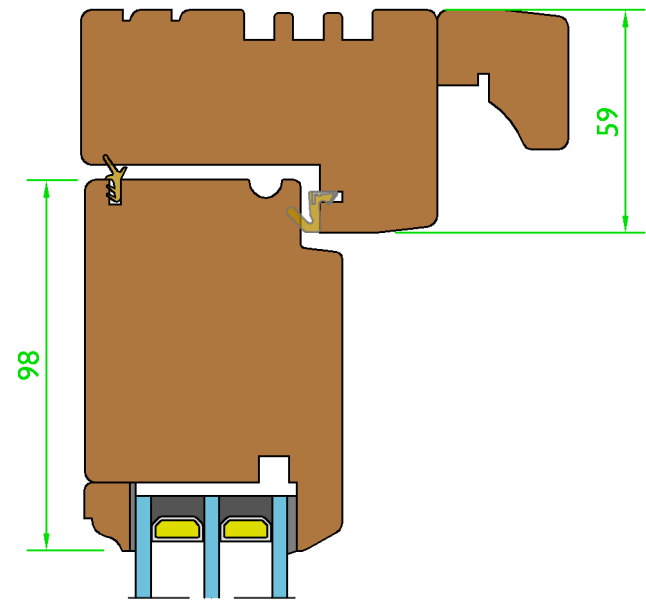
Frame With Head Drip Option - (Scale 1:2)
