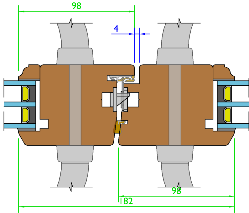
Section K-K - French Meeting Rail Options French Door Meeting - (Scale 1:2)
